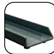
Shelf Deck Supports » 16 gauge steel » 2 1/2" Height » Adds capacity to shelf when bolted between double rivet beams
